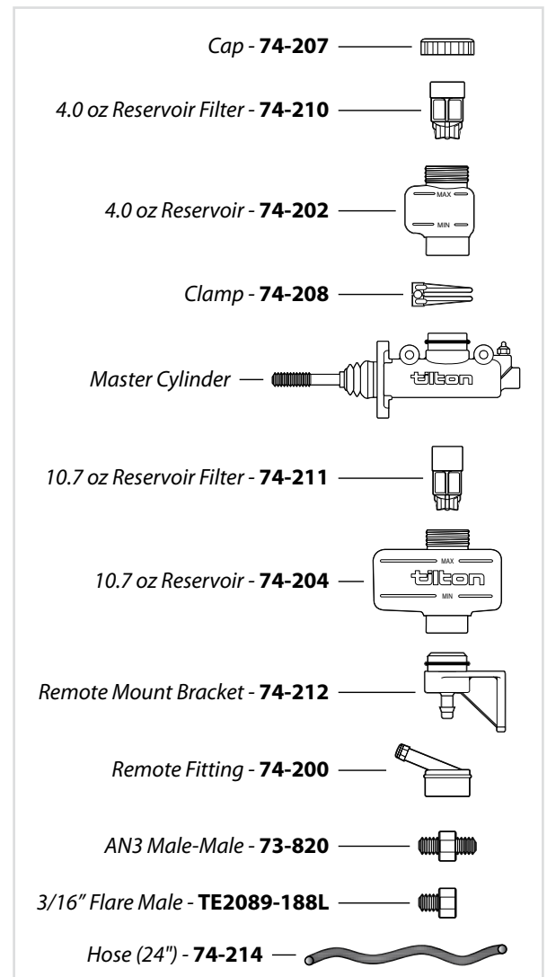
Diagram 1 - Master Cylinder Kit and Replacement Parts
